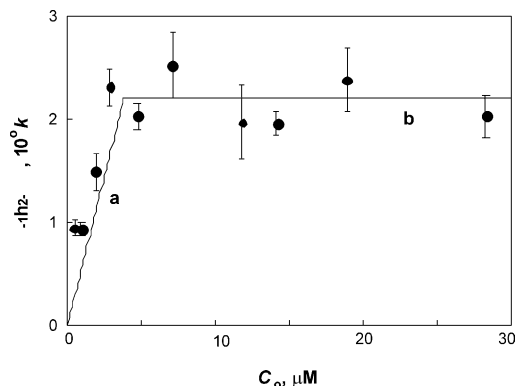
Figure 3. The plot of k_o against C_o for cleavage of Mb ( [Mb]_0 = 4.7 \mu\text{M} ) by Co(III) 1 at pH 7.5 and 37^\circ\text{C} (0.05 M buffer; addition of 0.5 M NaCl did not affect the rate data appreciably). Straight lines a ( C_o < S_o ) and b ( C_o \geq S_o ) stand for v_o/S_o ( v_o : initial velocity) and k_o , respectively, as predicted by Michaelis–Menten scheme under the condition of C_o \gg K_m .
