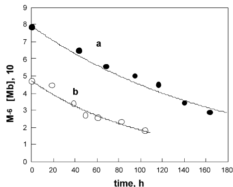
Figure 2. Decrease in [Mb] during incubation of Mb with Cu(II) 1 (●; curve a, [Mb]_o = 7.9 \mu\text{M} , [Cu(II)\mathbf{1}]_o = 2.0 \mu\text{M} ) or Co(III) 1 (○; curve b, [Mb]_o = 4.7 \mu\text{M} , [Co(III)\mathbf{1}]_o = 0.47 \mu\text{M} ) at pH 7.5 and 37 °C. The curves were obtained as indicated in the text: k_o = 5.7 \times 10^{-3} \text{ h}^{-1} for curve a and 9.4 \times 10^{-3} \text{ h}^{-1} for curve b.
