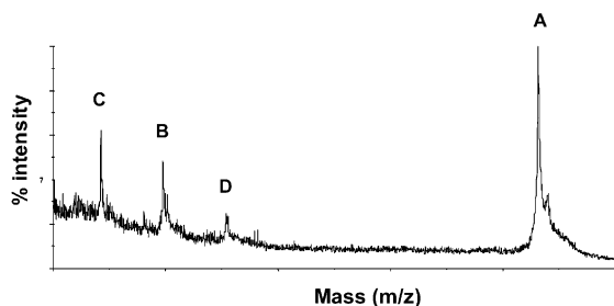
Figure 7. MALDI-TOF MS taken after incubation of Mb (9.8 \mu M) with Co(III) 7 (9.8 \mu M) at pH 7.5 and 37 °C for 96 h. Mass values ( m/z ) are 16953 (A), 16953/2 (B), 7068 (C), and 9888 (D); A and B are peaks for Mb and C and D are for proteins formed by cleavage of Mb.
