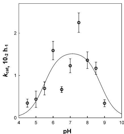
Figure 4. pH dependence of k_{\text{cat}} for cleavage of Mb by Co(III) 1 at 37^\circ\text{C} . The bell-shaped curve was obtained by analyzing the data by treating the Co(III) 1 –Mb complex as a diprotic acid ( pK_{a1} = 5.5 , pK_{a2} = 8.7 ) and by assuming that the monoprotonated species is reactive.
