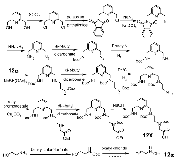
Scheme 6. Synthesis of 12X .
