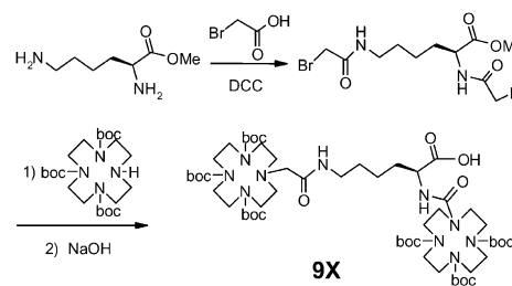
Scheme 3. Synthesis of 9X .
