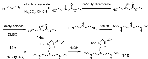
Scheme 8. Synthesis of 14X .
