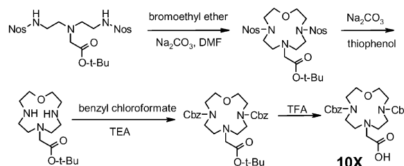
Scheme 4. Synthesis of 10X .
