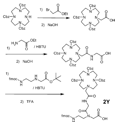
Scheme 1. Synthesis of 2Y .
