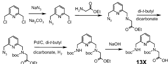
Scheme 7. Synthesis of 13X .
