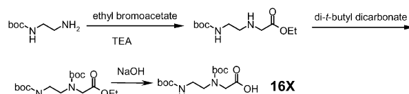
Scheme 10. Synthesis of 16X .
