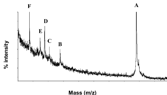
Figure 6. MALDI-TOF MS taken after incubation of Mb ( 12 \mu\text{M} ) with Co(III) 1 ( 3.5 \mu\text{M} ) at pH 6.0 and 37^\circ\text{C} for 85 h. Mass values ( m/z ) are 16953 (A), 9892 (B), 8909 (C), 16953/2 (D), 8045 (E), and 7074 (F); A and D are peaks for Mb (M.W. 16953) and two pairs (B/F and C/E) are for proteins formed by cleavage of Mb.
