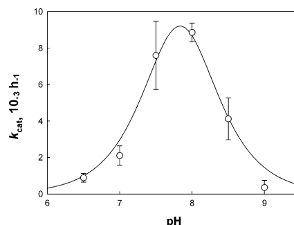
Figure 5. pH dependence of k_{\text{cat}} for cleavage of Mb by Co(III) 10 at 37^\circ\text{C} . The bell-shaped curve was obtained by treating the Co(III) 10 –Mb complex as a diprotic acid ( pK_{a1} = 7.4 , pK_{a2} = 8.3 ) and by assuming that the monoprotonated species is reactive.
