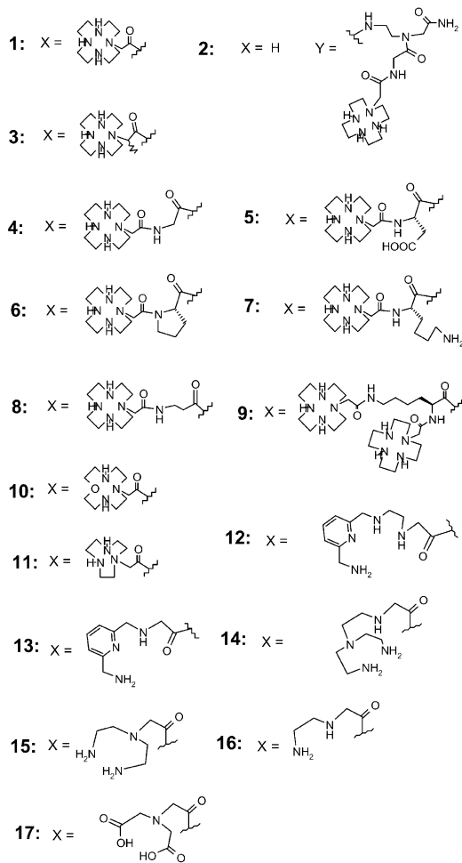
Figure 1. Structures of 1–17 .
