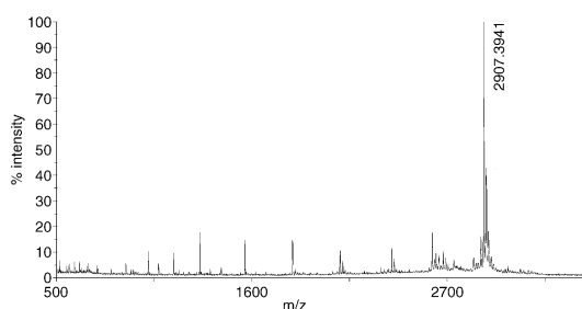
Figure 8. MALDI-TOF MS of Co(III) 1 ; m/z 2907.39 ( M+H ) + (C 111 H 153 N 64 O 25 S 2 Co calcd 2906.91).
